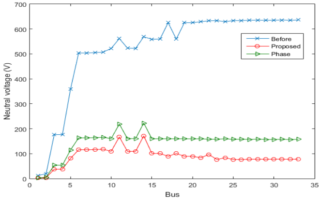
Fig. 5. Neutral voltage (case 2).
