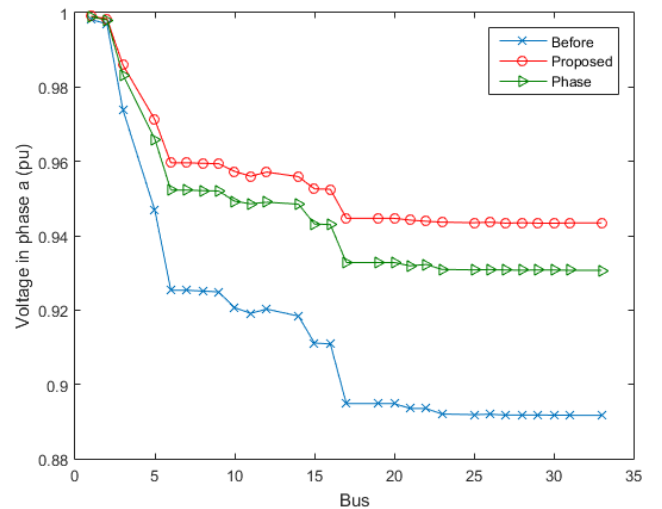
Fig. 4. Voltage in phase a (case 2).
