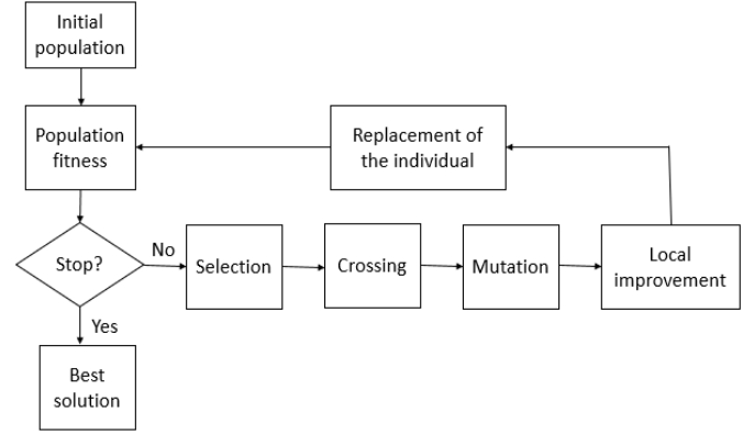
Fig. 3. Flowchart of the optimization algorithm.
