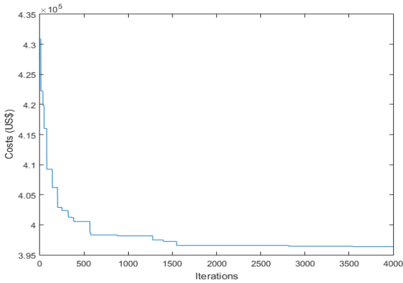
Fig. 7. Algorithm convergence for the phase method.
