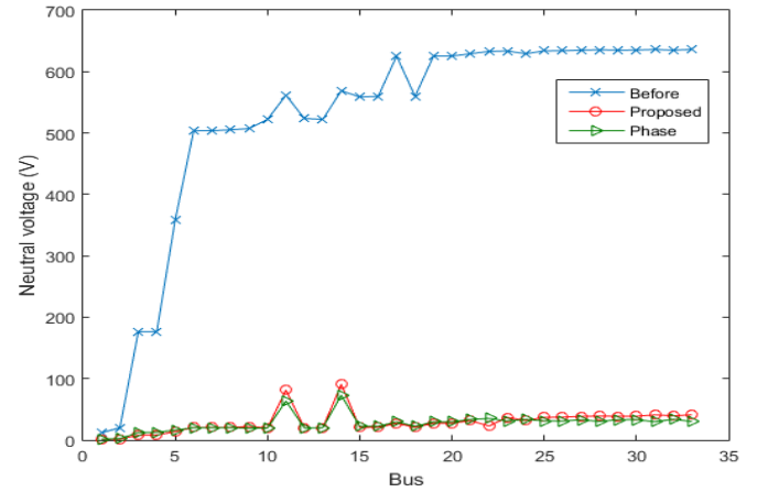
Fig. 9. Neutral voltage (case 3).
