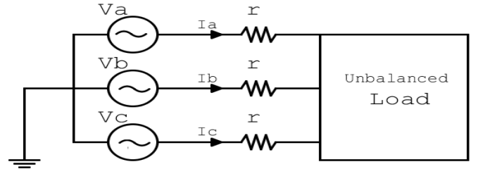
Fig. 1. Unbalanced and symmetrical three-phase system.
