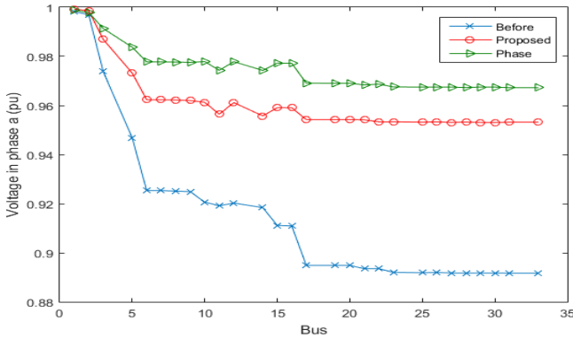
Fig. 10. Voltage in phase a (case 4).
