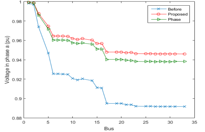
Fig. 8. Voltage in phase a (case 3).
