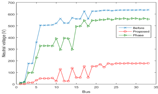
Fig. 11. Neutral voltage (case 4).
