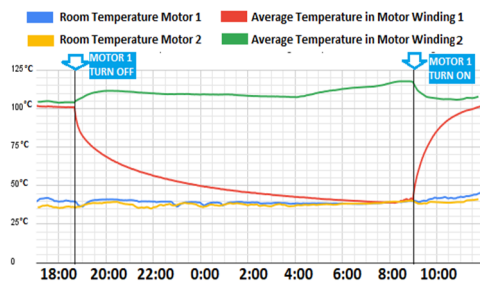
Figure 8: Temperature variation in one engine due to the state of the other engine.
