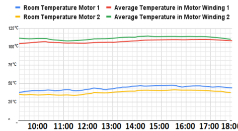
Figure 7: Comparison between ambient temperature and internal temperature of both engines simultaneously.
