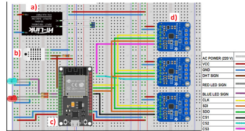
Figure 2: Assembly of the electronic circuit. Where is shown: (a) power supply; (b) outdoor temperature and humidity sensor; (c) ESP32 controller; (d) MAX 31865 digital converter.
